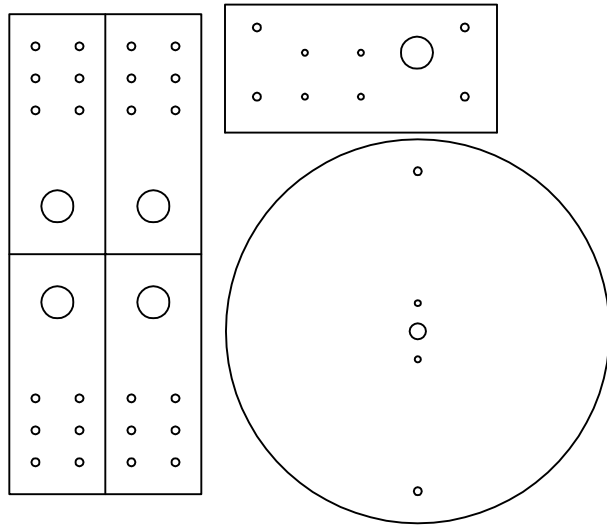
Structure for central gear and attachment to ceiling
