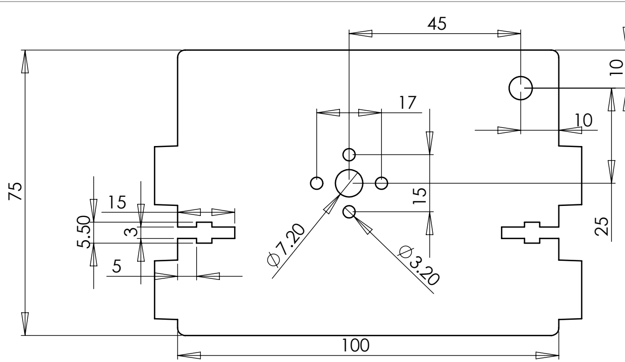
Front Plate with Gearmotor Mount
