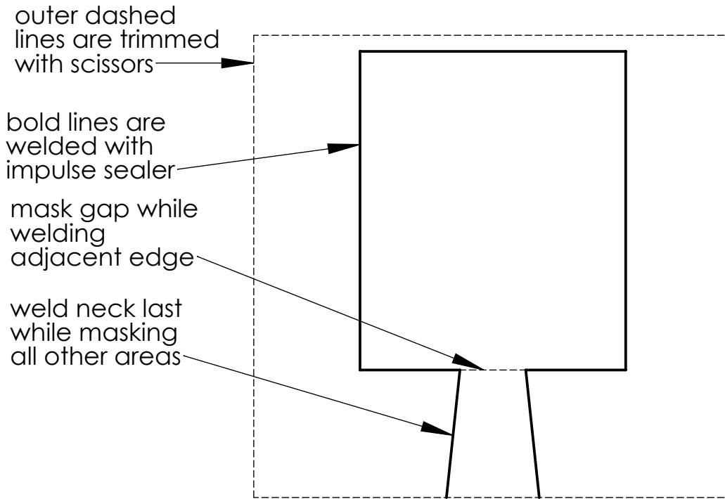
Basic pouch actuator. The trim lines are wide to allow for attaching cardboard stiffeners to form a hinge joint.
