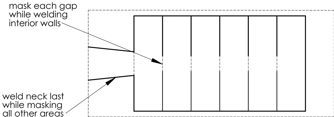
Linear contraction actuator. The trim lines may be widened as needed to allow for attaching to other materials.
