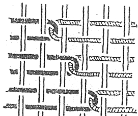
diagonal interlock—common weft
