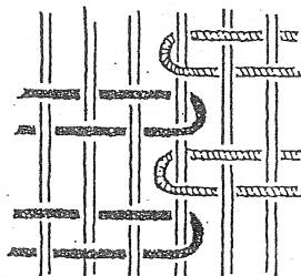
straight interlock—common warp
